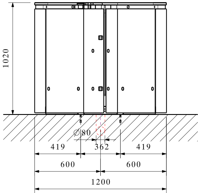
VIEW X-X & Y-Y
